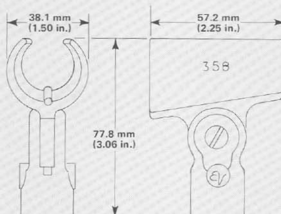
FIGURE 1 - Dimensions
